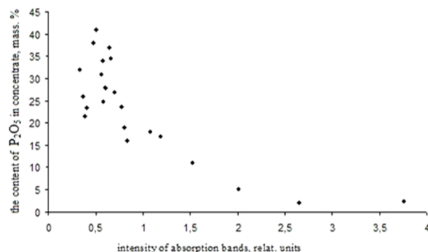
Fig. 6. The relationship between the intensity of the absorption band of the group (\text{CO}_3)^{2-} in the IR spectra of apatite of the Kovdor deposit in the region of 870 \text{cm}^{-1} and the content of \text{P}_2\text{O}_5 in the apatite concentrate.
