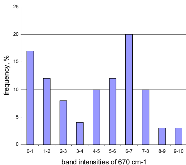
Fig. 3. Histogram of the distribution of quantities band intensities of 670 cm^{-1} in the spectra of mono-baddeleyite fractions of the Kovdor field.
