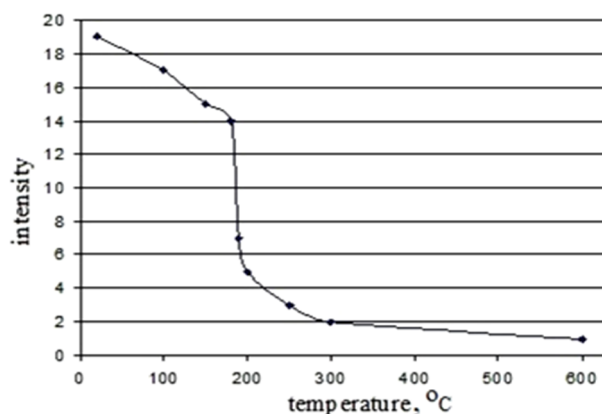
Fig. 7. Changes in the intensity of absorption bands in the region of 3600-3200\text{ cm}^{-1} in the IR spectra of goethite of the Skelevat iron ore deposit under temperature exposure.
