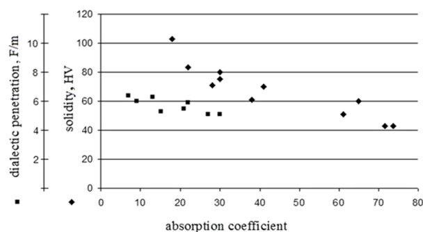
Fig. 1. The relationship between the intensity of the bands of 3550 cm^{-1} and 3400 cm^{-1} of the IR spectrum of the phlogopite of the Kovdor deposit and its physical properties.
