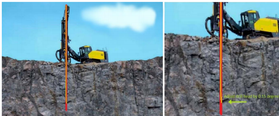
Fig. 2. Augmented drill hole with indicated deflection on the drill head
