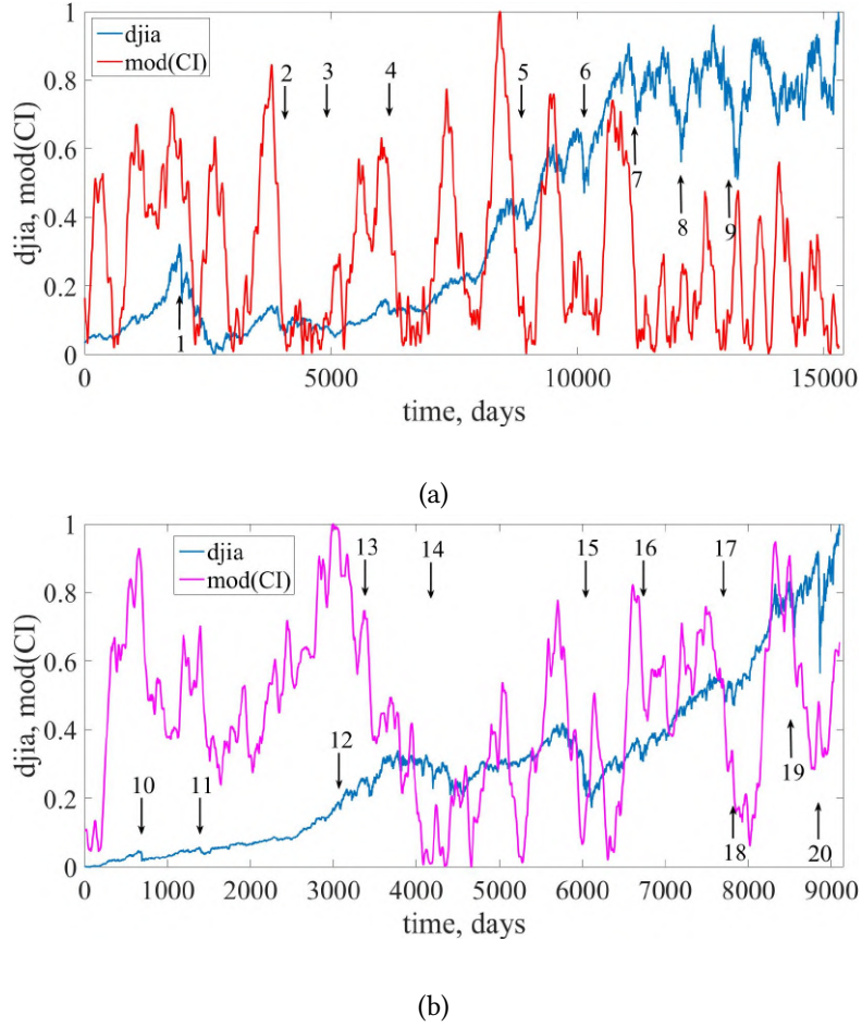
Figure 4: Dynamics of Costa's index for first (a) and second (b) periods of DJIA time series.
