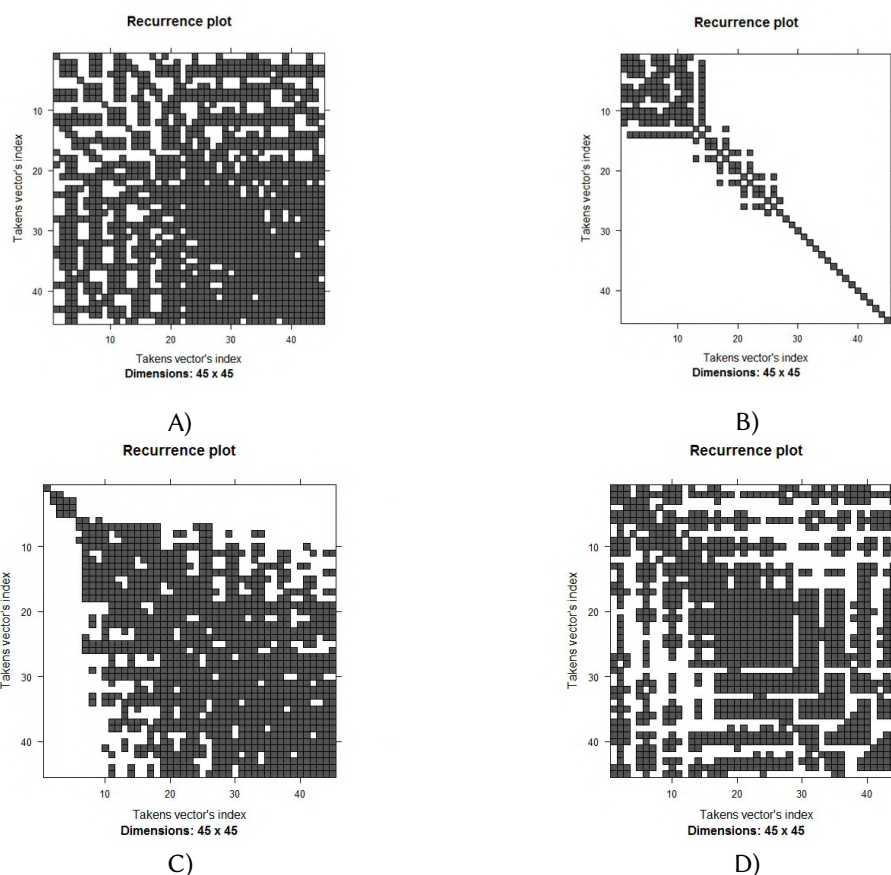
Figure 2: Recurrence plot of the behavior of digital economy agents (frequency of online requests “bitcoin” according to Google Trends in Ukraine): A) July 12, 2015 – October 02, 2016, B) October 09, 2016 – December 31, 2017, C) January 07, 2018 – March 31, 2019, D) April 07, 2019 – June 28, 2020.
